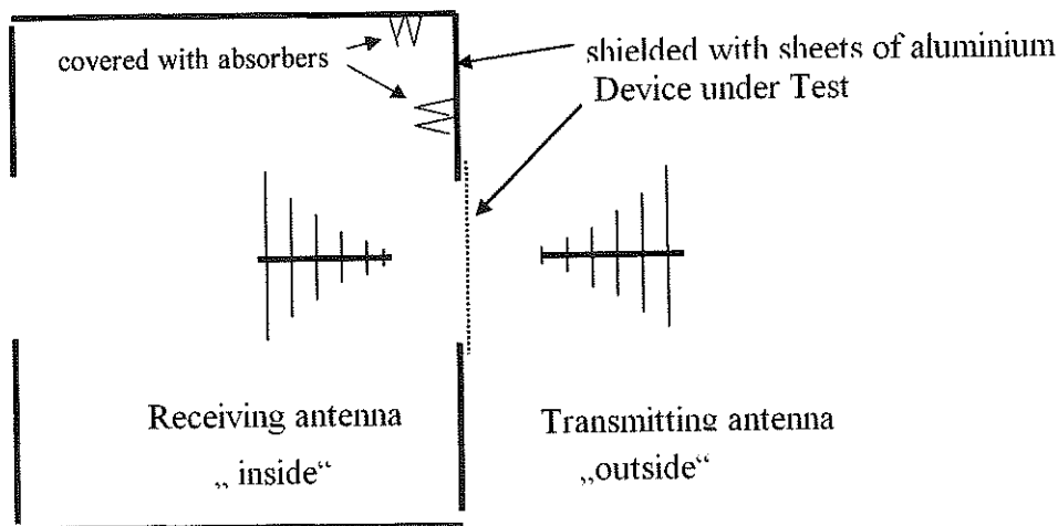
Setup for Shielding Measurements
